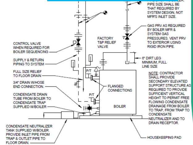
CONDENSING BOILER PIPING DETAIL
